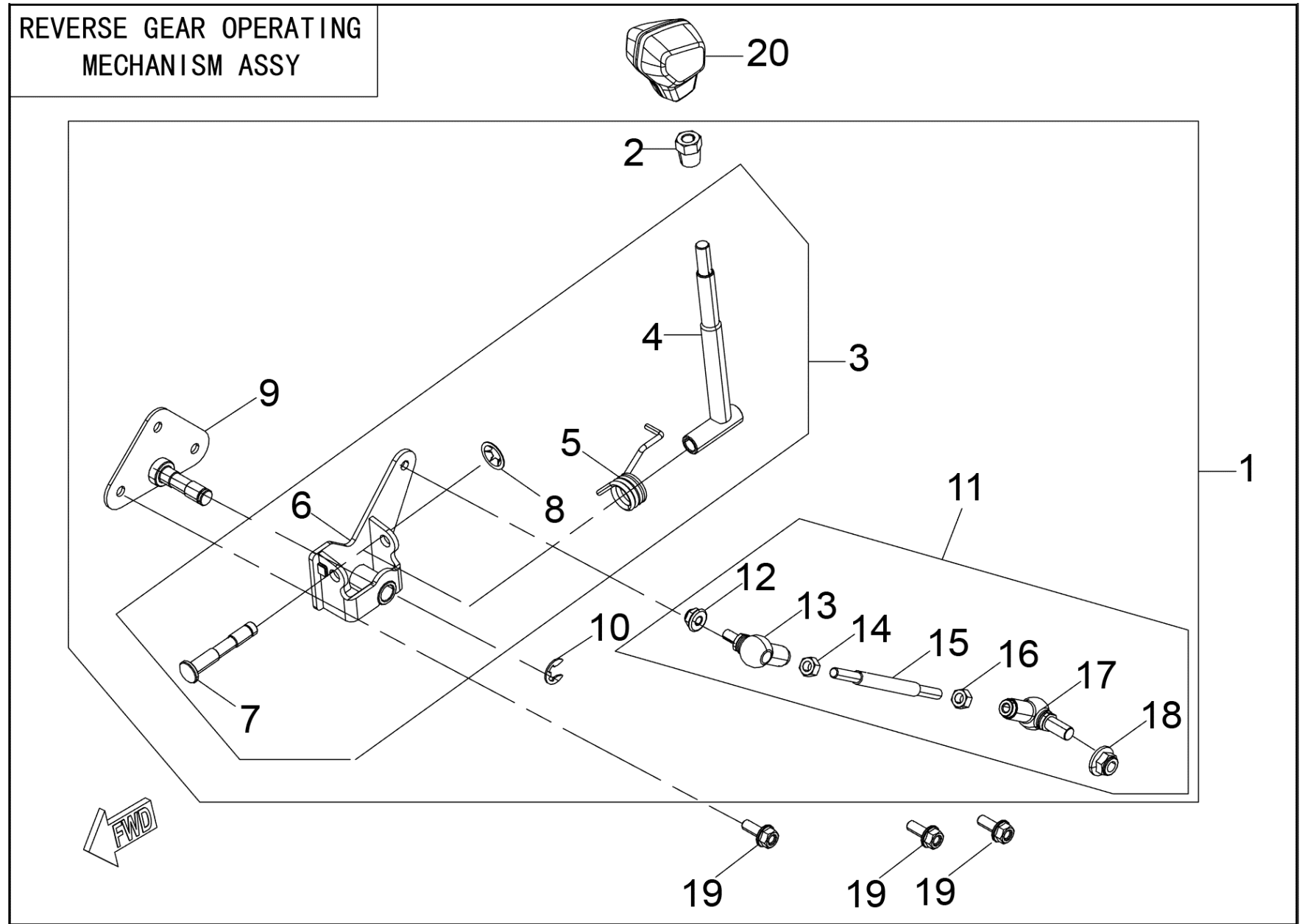
FIGUR 5 – GEARSTANG
