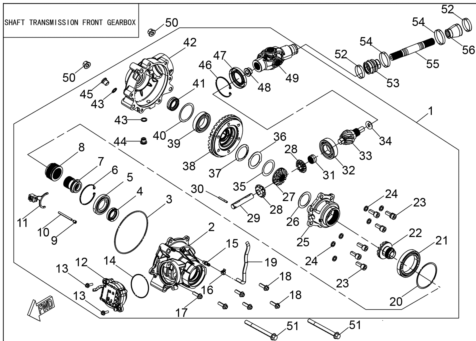
FIGUR 7 – TRANSMISSION (1)
