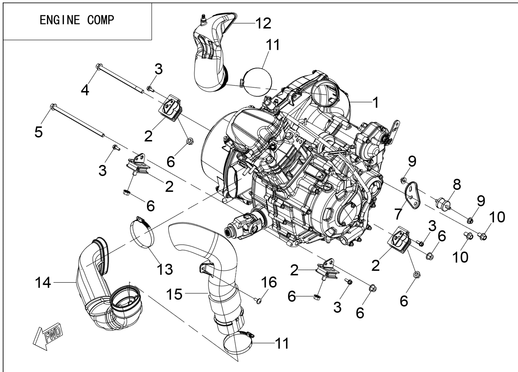
FIGUR 6 – MOTOR
