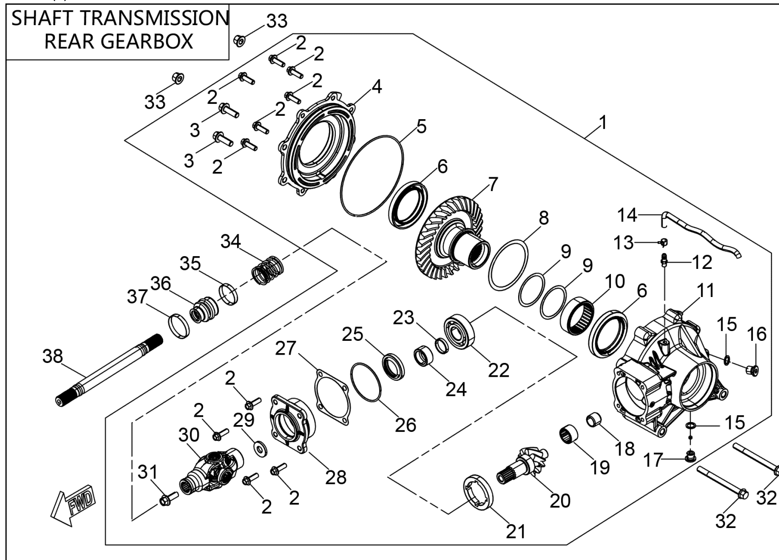
FIGUR 8 – TRANSMISSION (2)
