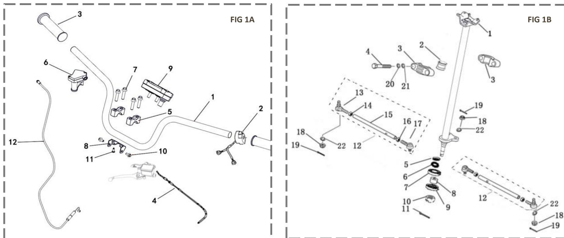
FIGUR 1 – STYR / HANDLEBAR
